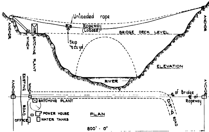
Fig. 276.—Arrangement of Plant with Overhead Ropeway.
